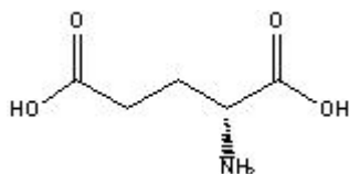
D-Glutamic Acid
