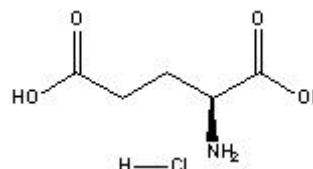
L-Glutamic Acid
